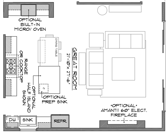
KITCHEN HALF ISLAND/ TABLE OPTION B
